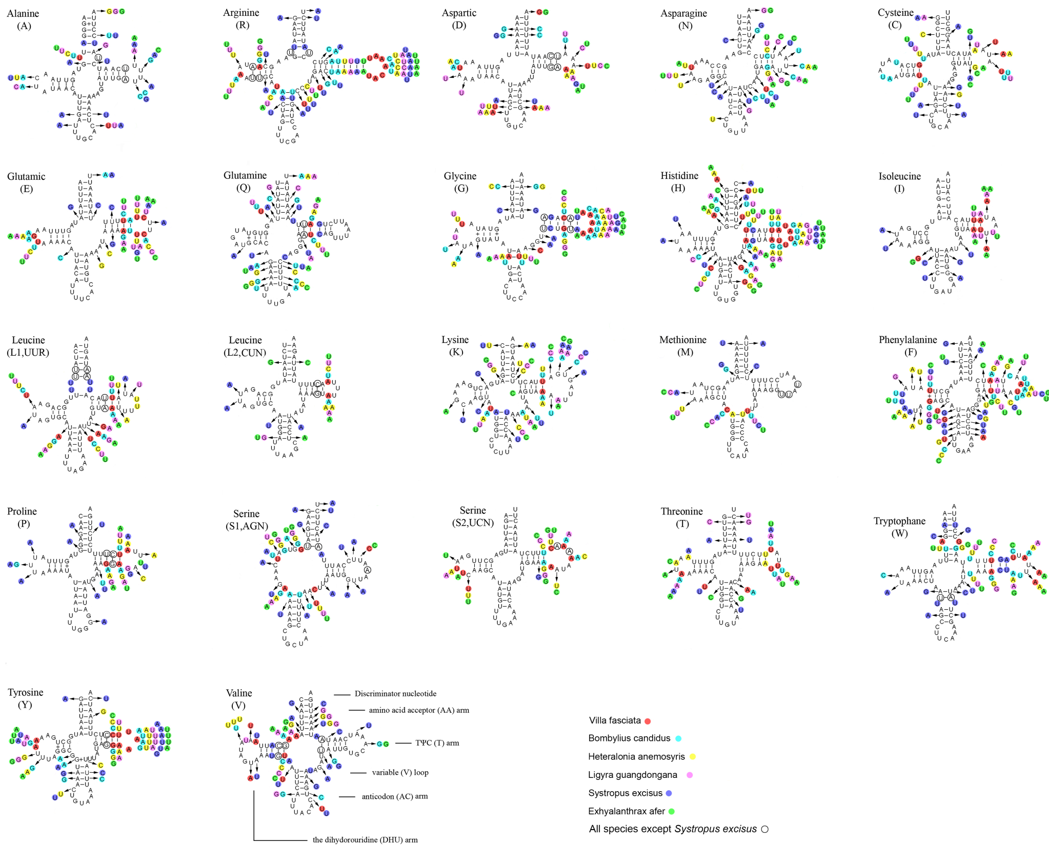
Fig. S1. Inferred secondary structures of 22 tRNAs in the species sequenced. The tRNAs are identified by the abbreviations of their corresponding amino acids. Dash (—) indicates Watson-Crick bonds and symbol (+) indicates GU bonds.
