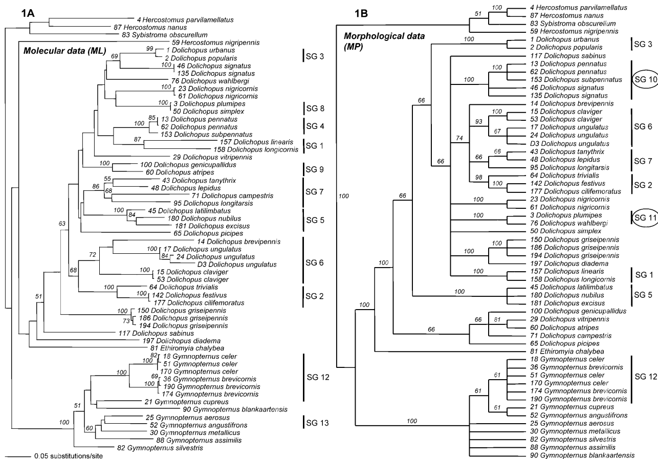
Fig. 1. A – ML tree from 100 bootstrap replicates, obtained from COI and Cyt-b combined sequences ( -Ln = 15925.39419 ). Bootstrap support values higher than 50% are indicated above branches. B – MP 50% majority rule consensus tree of 633 equally parsimonious trees (length = 98, consistency index = 0.418, retention index = 0.820, rescaled consistency index = 0.343, homoplasy index = 0.582) obtained from 32 morphological characters. Species groups (SG) refer to Table 4; encircled SGs only supported by morphological data.
