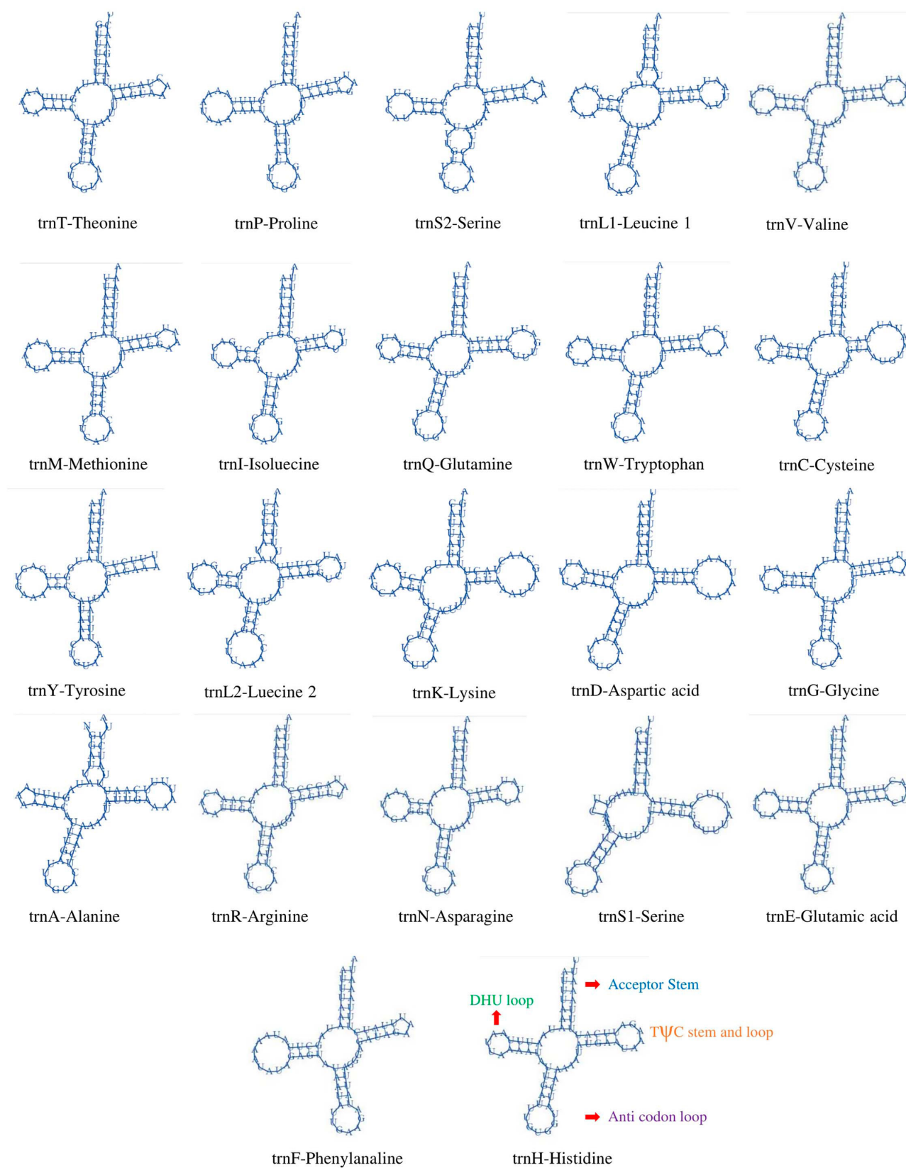
Fig. S3. Putative secondary structures of 22 tRNAs in mitochondrial genome of L. dorsigera .
