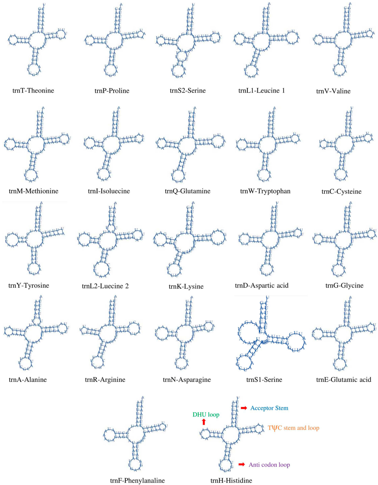
Fig. S2. Putative secondary structures of 22 tRNAs in mitochondrial genome of H. bolinoides .
